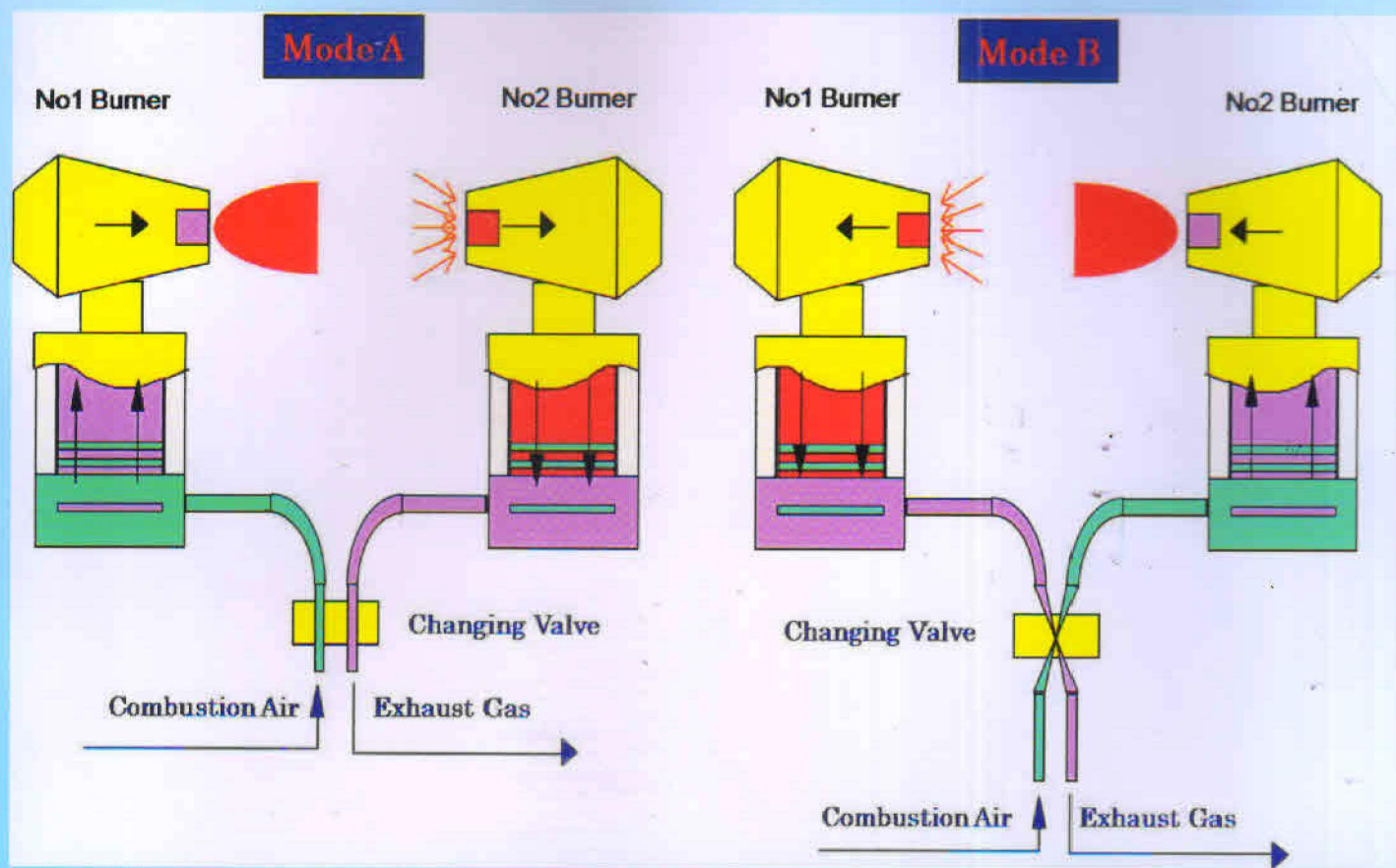
Control logic of regenerative burner system
